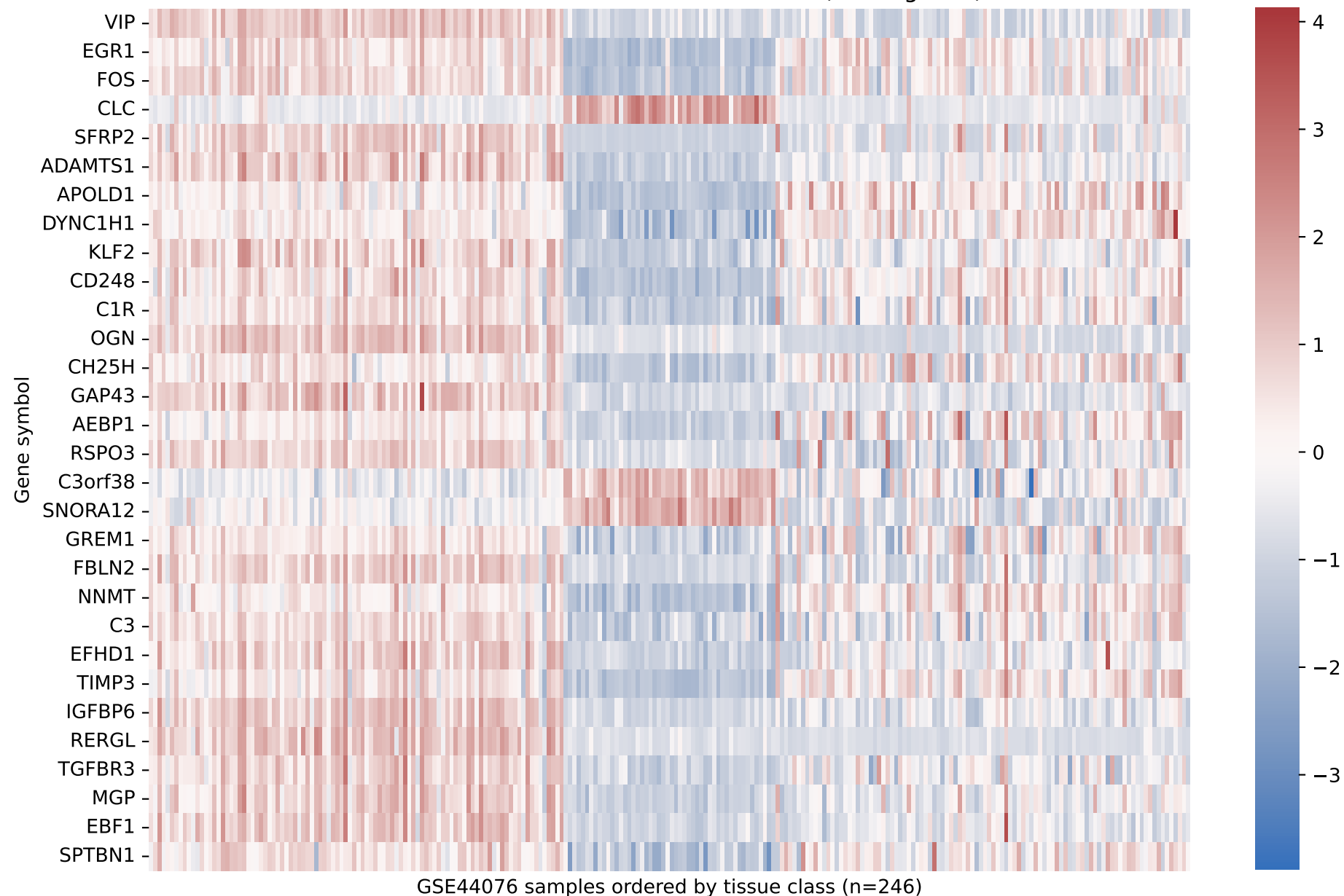
Raw-CEL field-cancerization candidates (n=30 genes)
