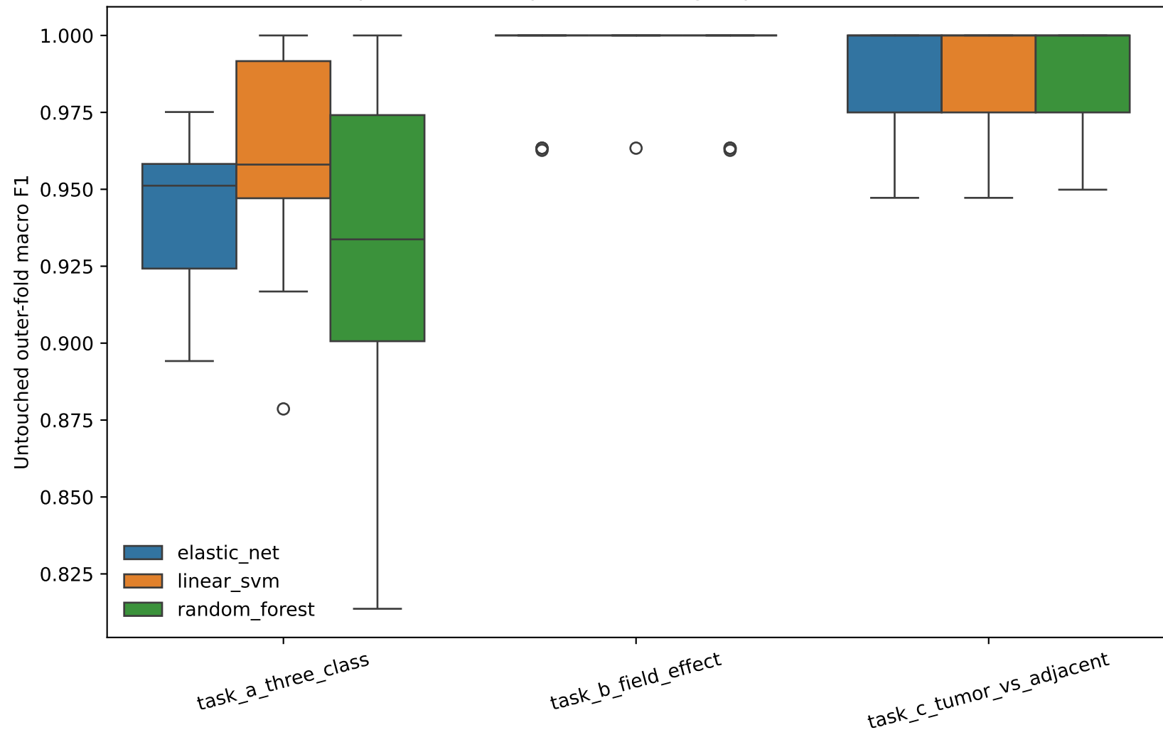
Repeated nested patient/donor-group cross-validation
