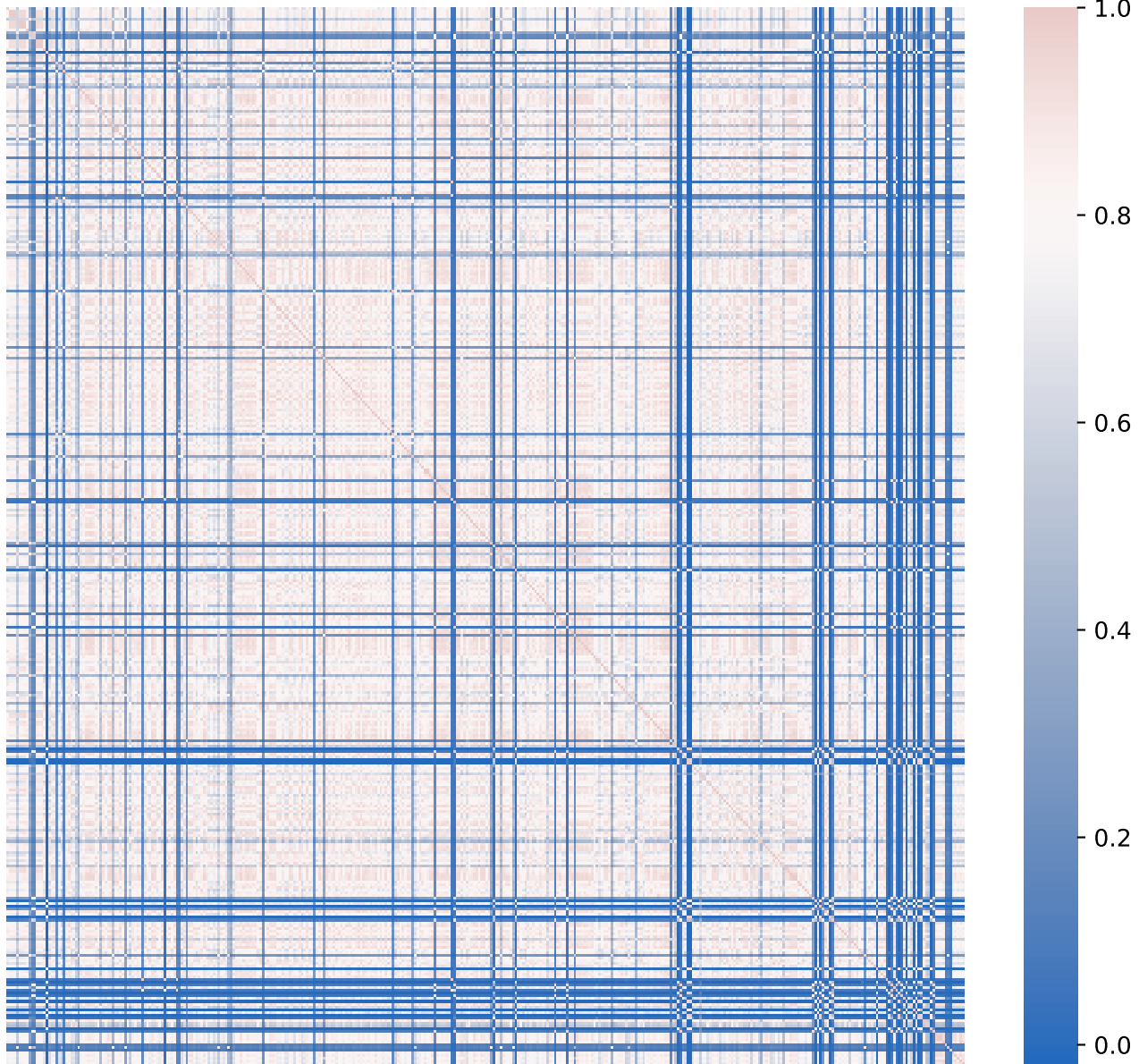
GSE41258: sample correlation (top variable genes)
