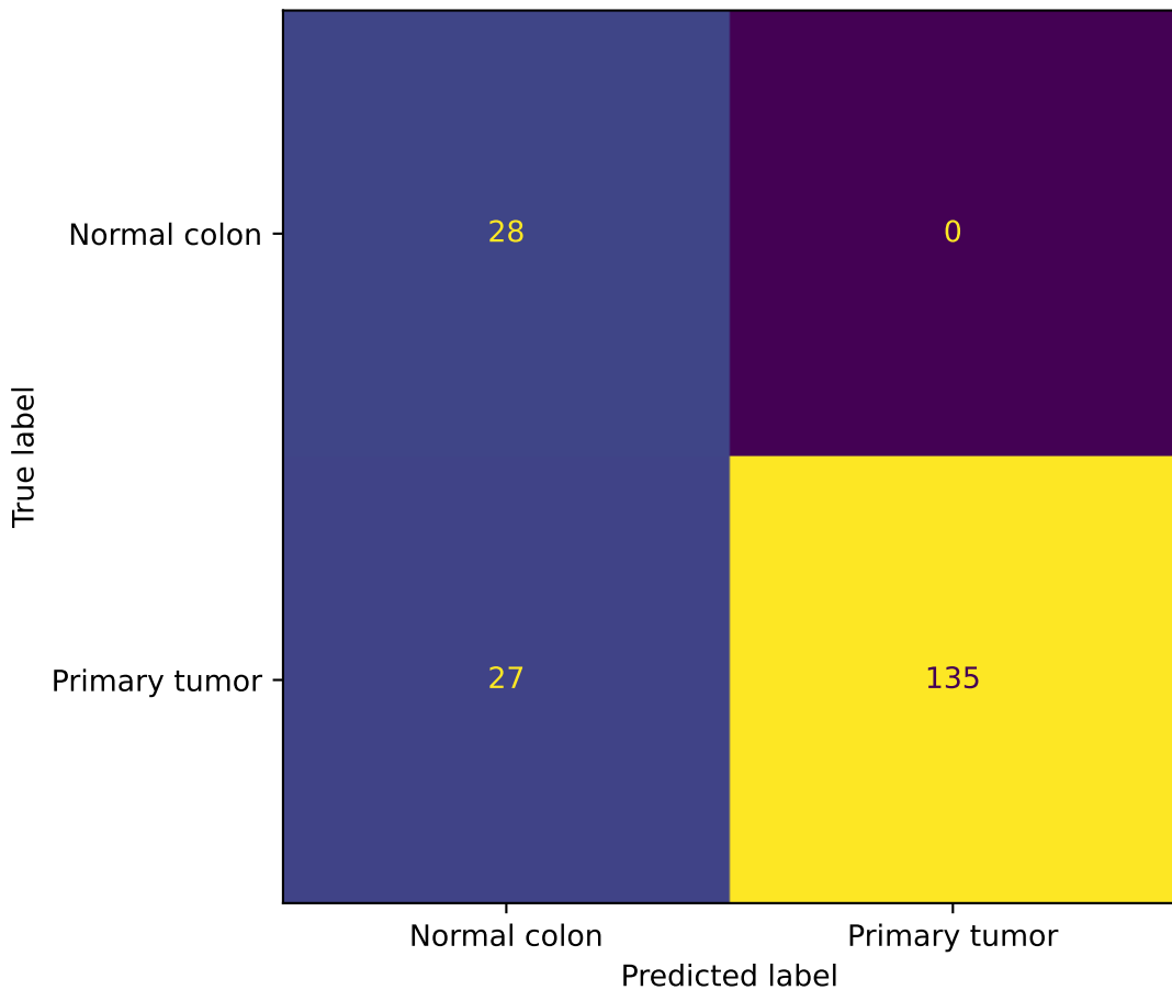
External confusion matrix (n=190)
