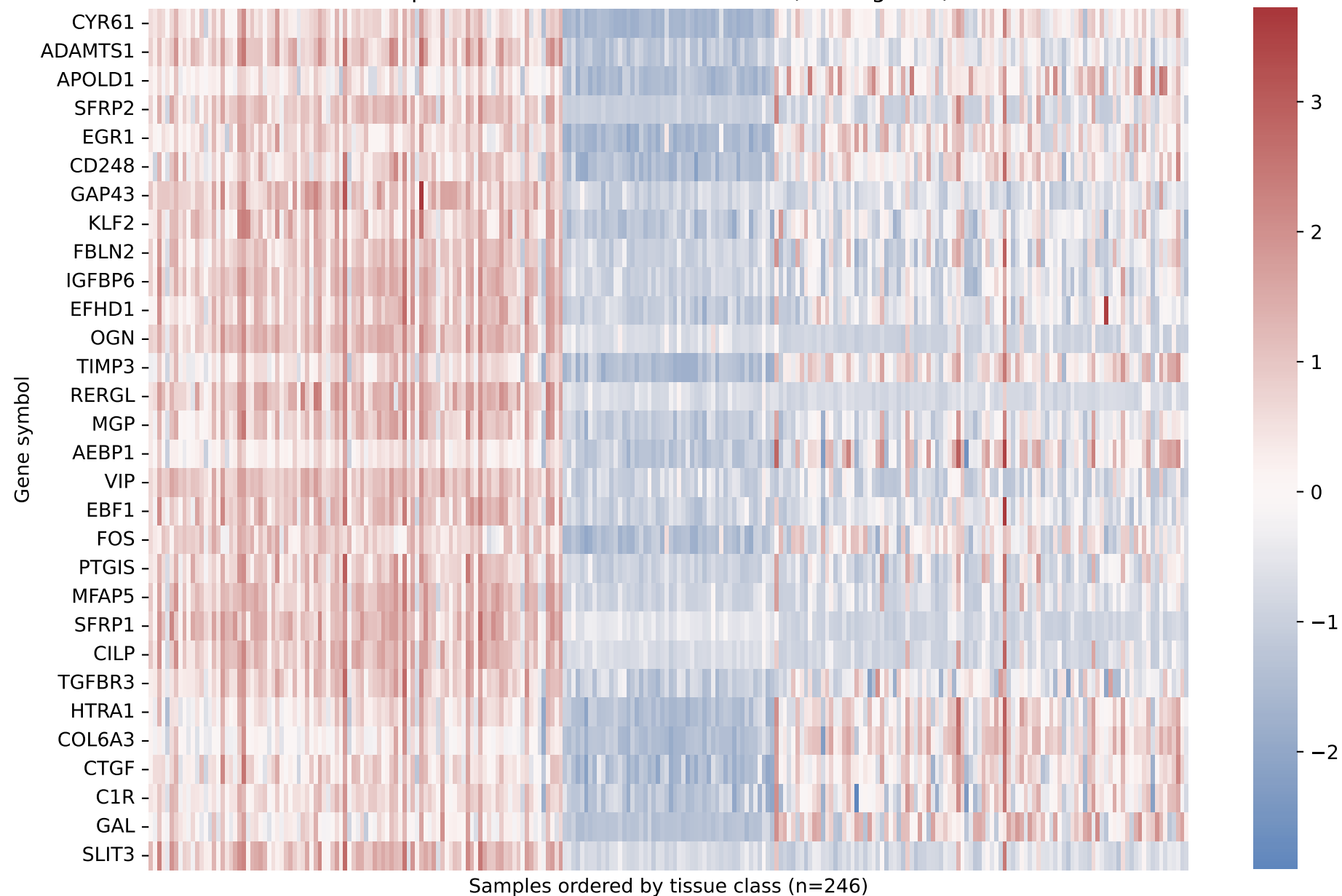
Top field-cancerization candidates (n=30 genes)
