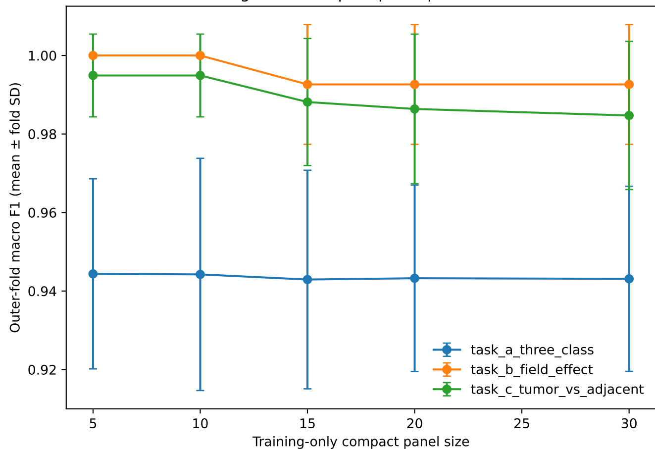
Leakage-safe compact-panel performance
