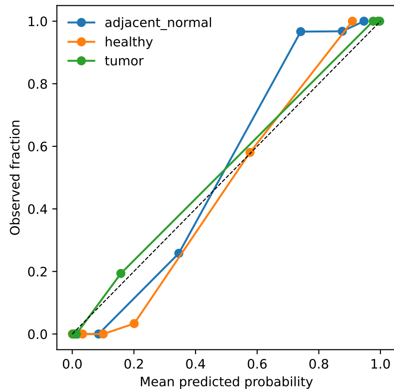
One-vs-rest calibration
