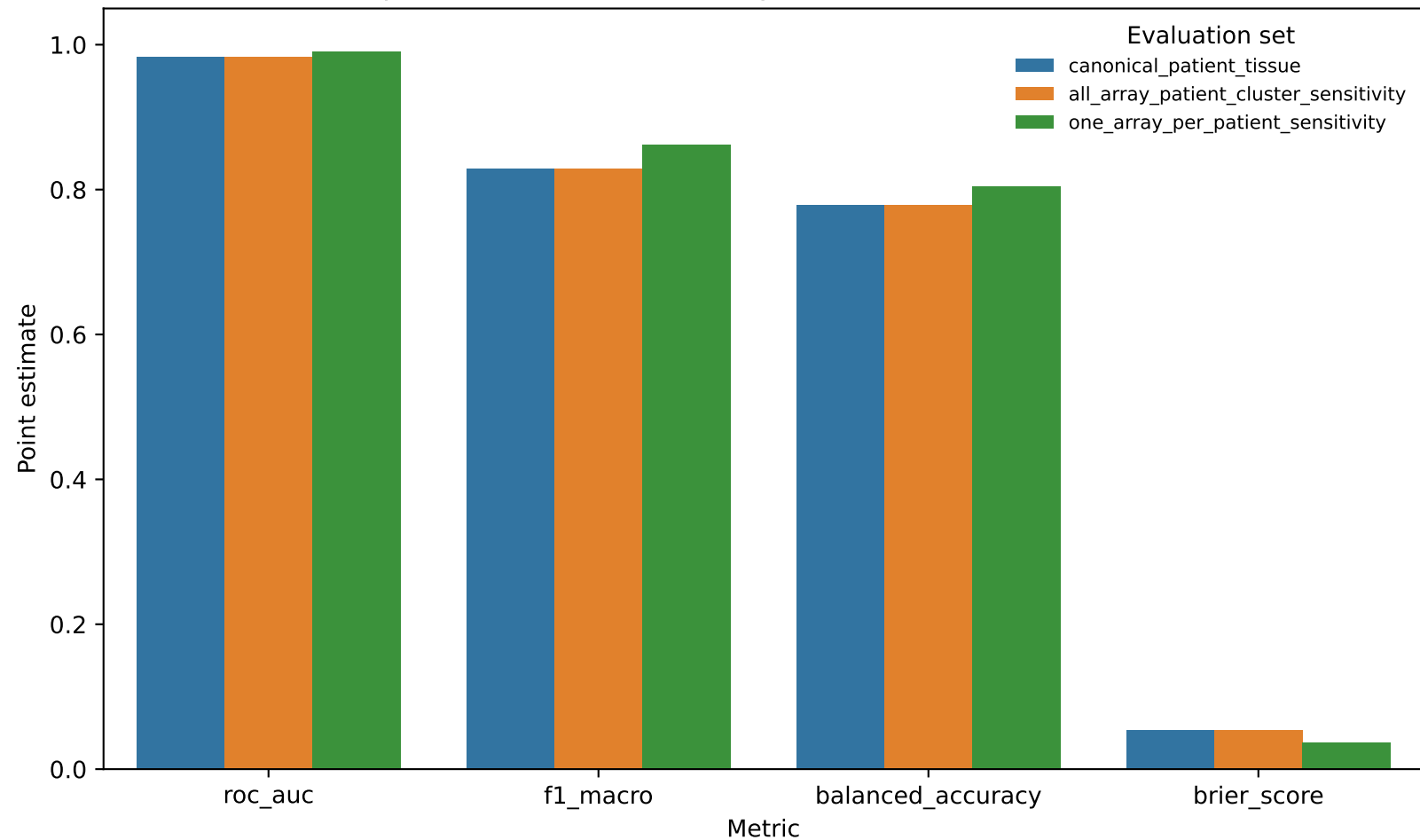
External patient-structure sensitivity at the GSE44076-locked threshold
