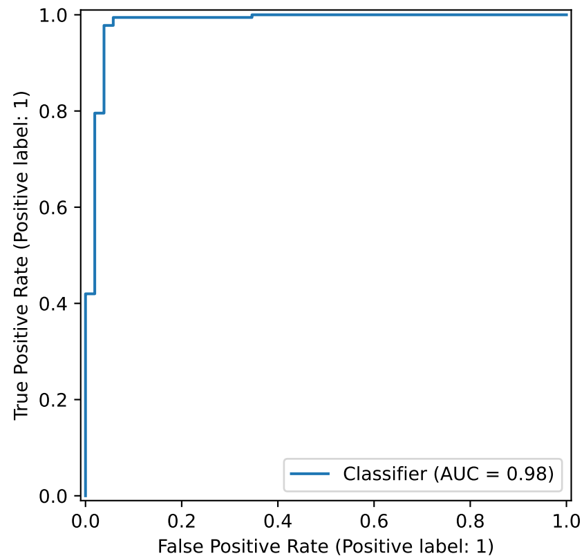
GSE41258 discrimination: canonical patient-tissue set
