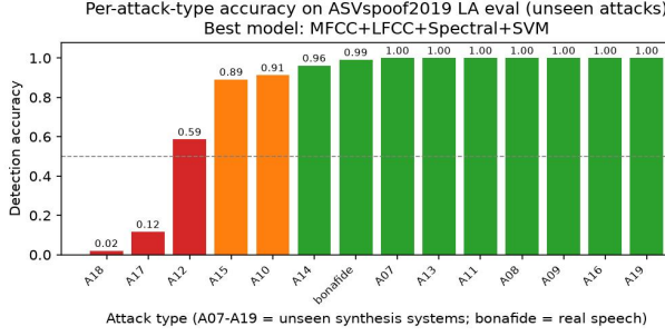
Fig. 2. Per-attack-type detection accuracy of the best model (MFCC+LFCC+Spectral+SVM) on unseen eval attacks.
