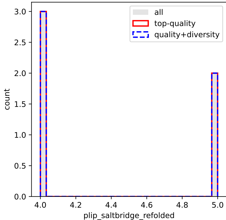
plip_saltbridge_refolded
