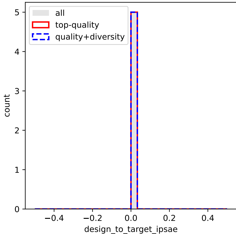
design_to_target_ipsae
