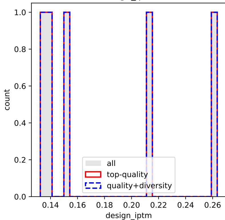
design_ipitm
