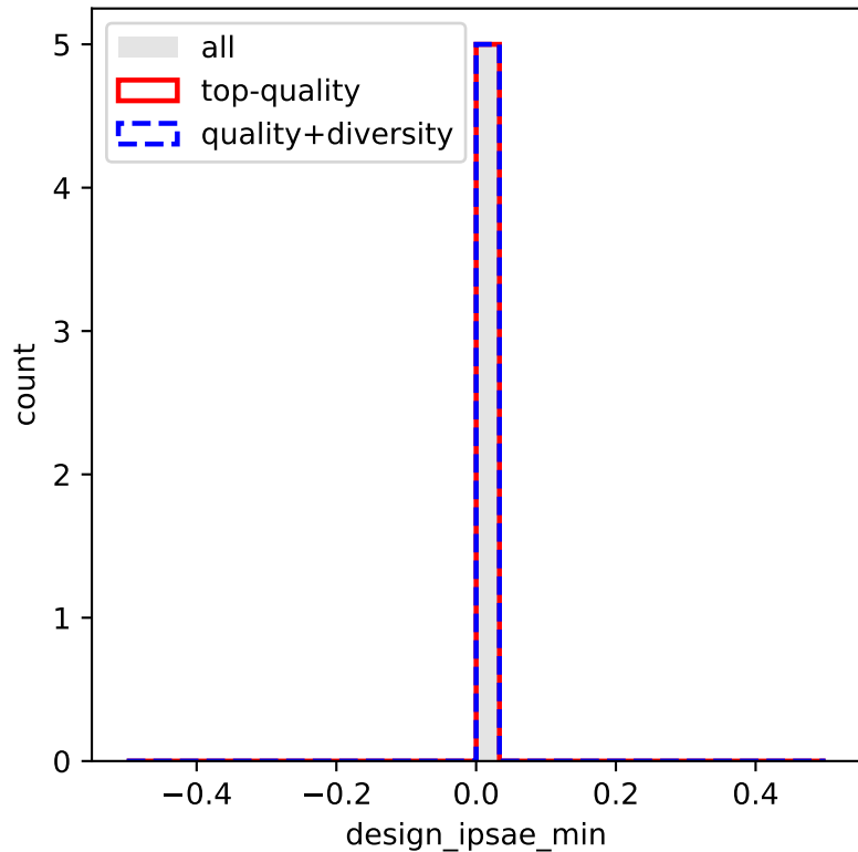
design_ipsae_min
