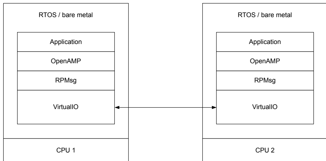
Figure 4. OpenAMP and RPMsg implementation layers
