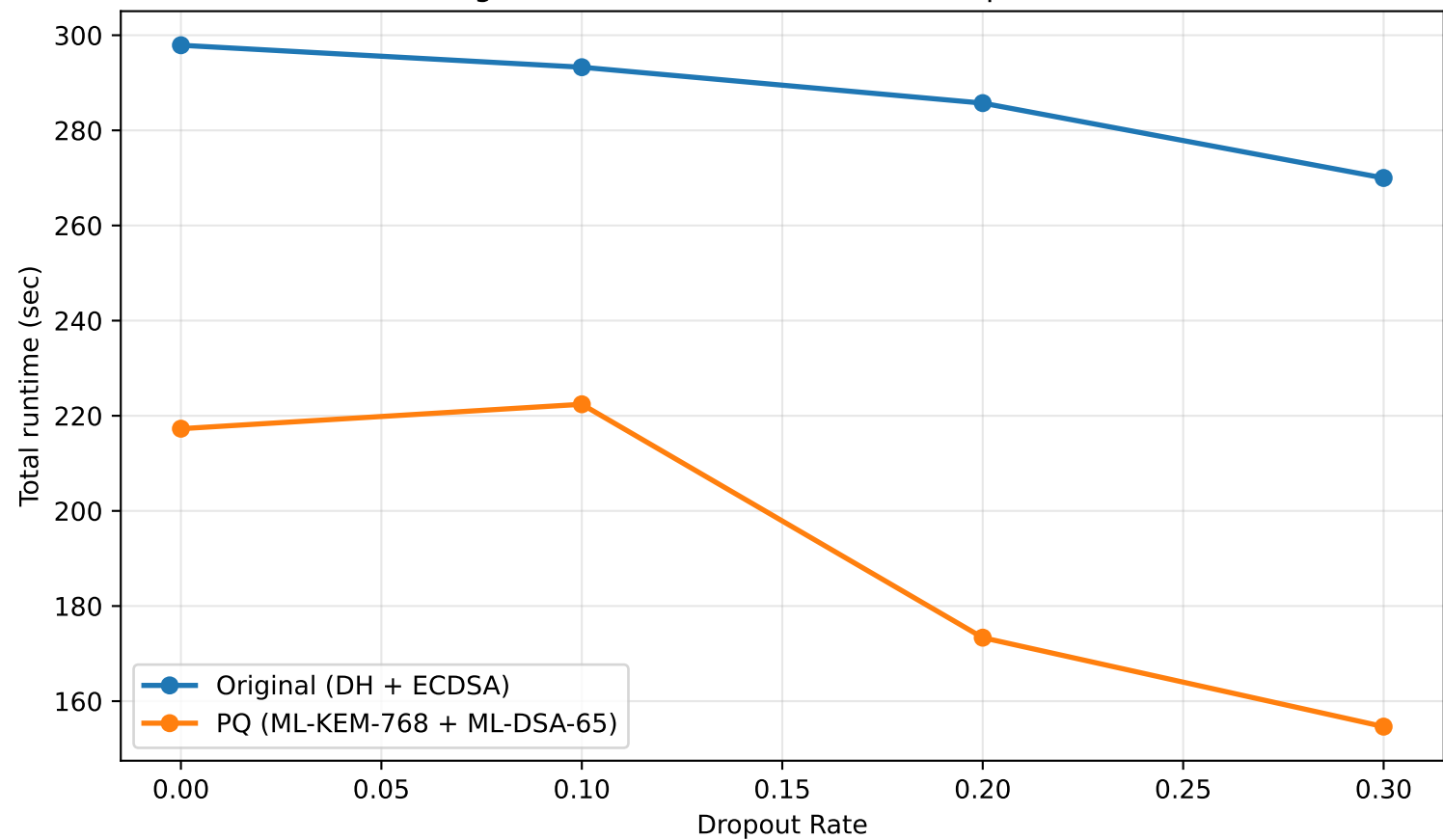
Original vs PQ: Total Runtime vs Dropout Rate
