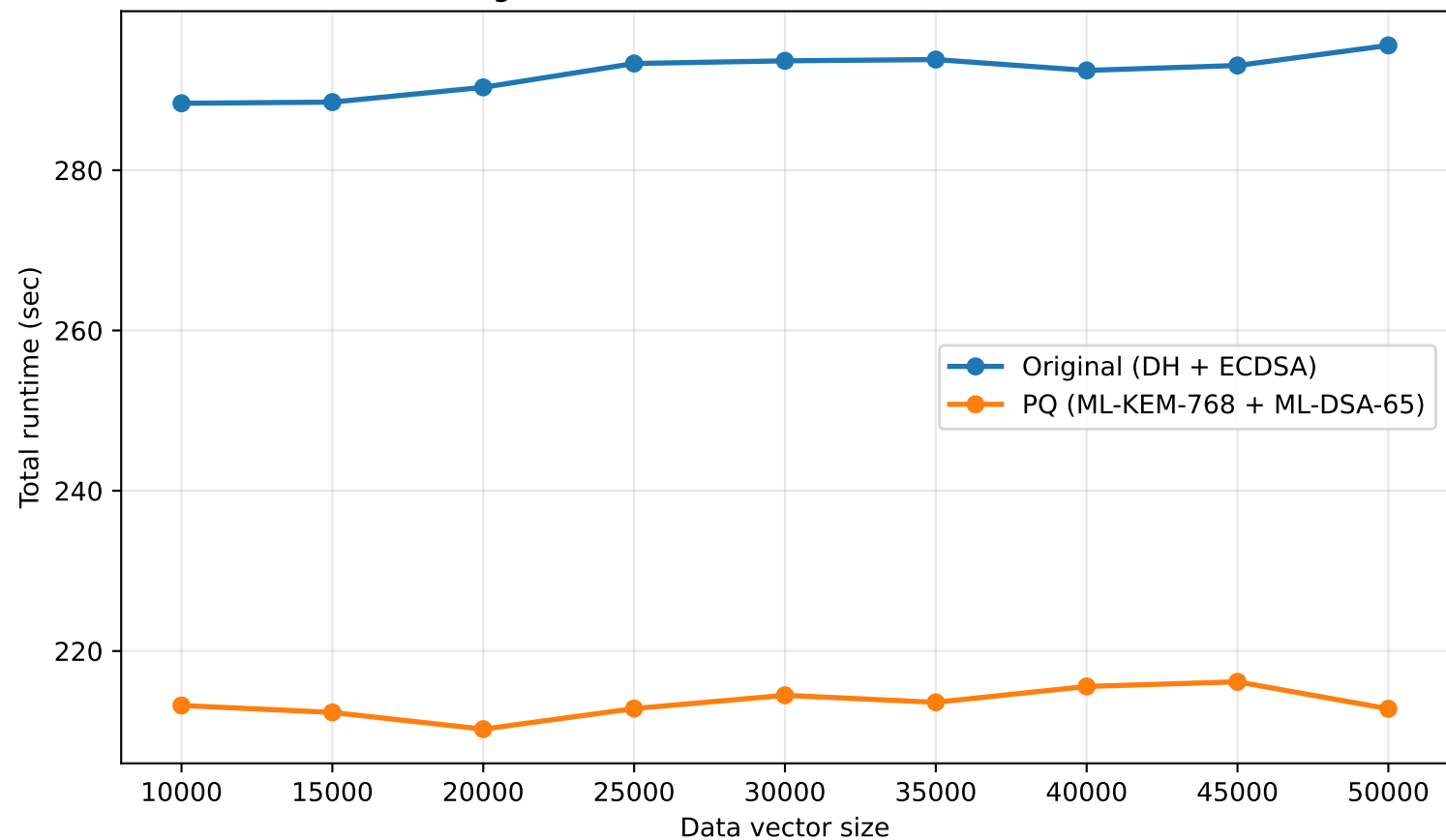
Original vs PQ: Total Runtime vs Vector Size
