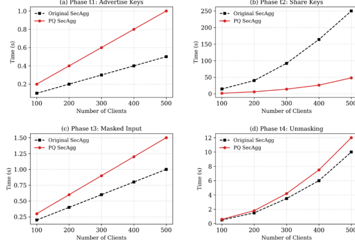
Fig. 2. Computational efficiency across protocol phases. Note the significant reduction in t_2 (Share Keys) for the PQ framework.
