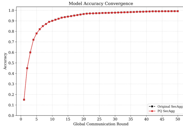
Fig. 5. Global model accuracy convergence. Both frameworks maintain identical utility during federated training.
