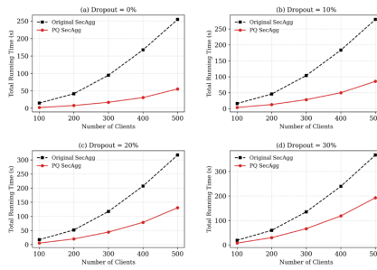
Fig. 3. Total latency vs. dropout rate.
