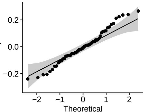
ENSG00000260878: R2 = 0.43, pval = 3e-07
