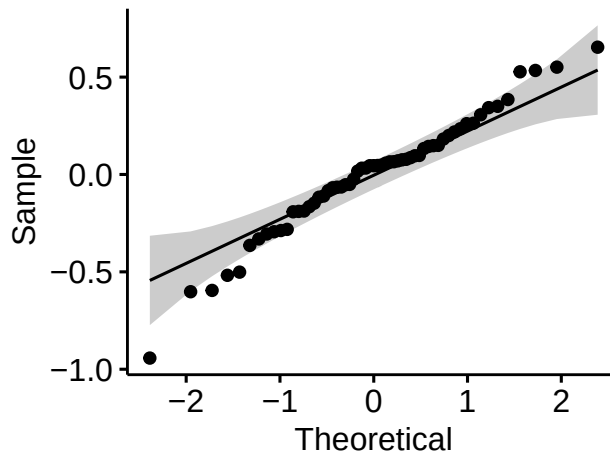
CREBZF: R2 = 0.43, pval = 3.7e-07
