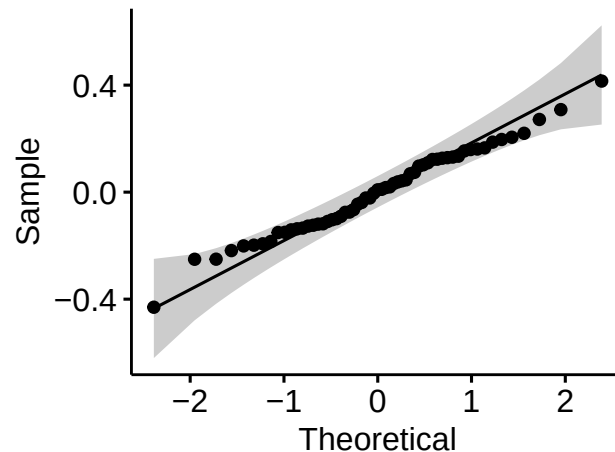
RAB14: R2 = 0.42, pval = 5e-07
