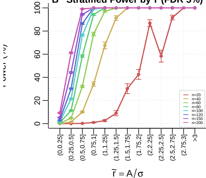
B Stratified Power by \tilde{r} (FDR 5%)
