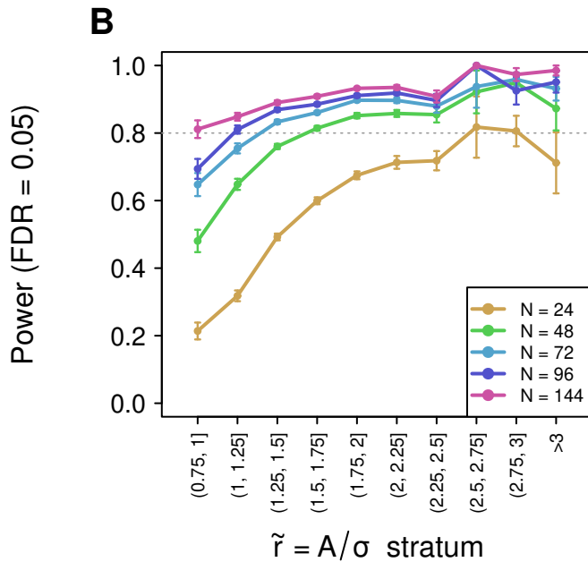
Stratified Power by \tilde{r}
