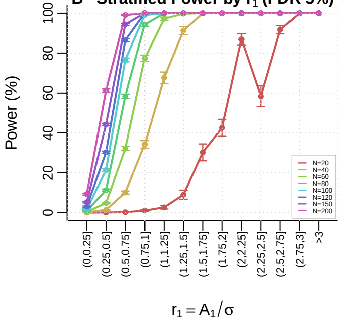
B Stratified Power by r_1 (FDR 5%)
