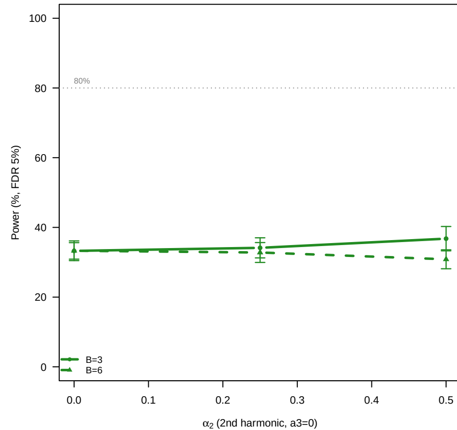
D1D2 (r~0.66) N=72: does B protect?
