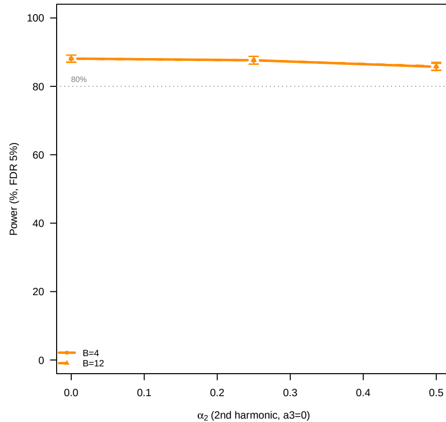
Baboon (r~1.7) N=48: does B protect?
