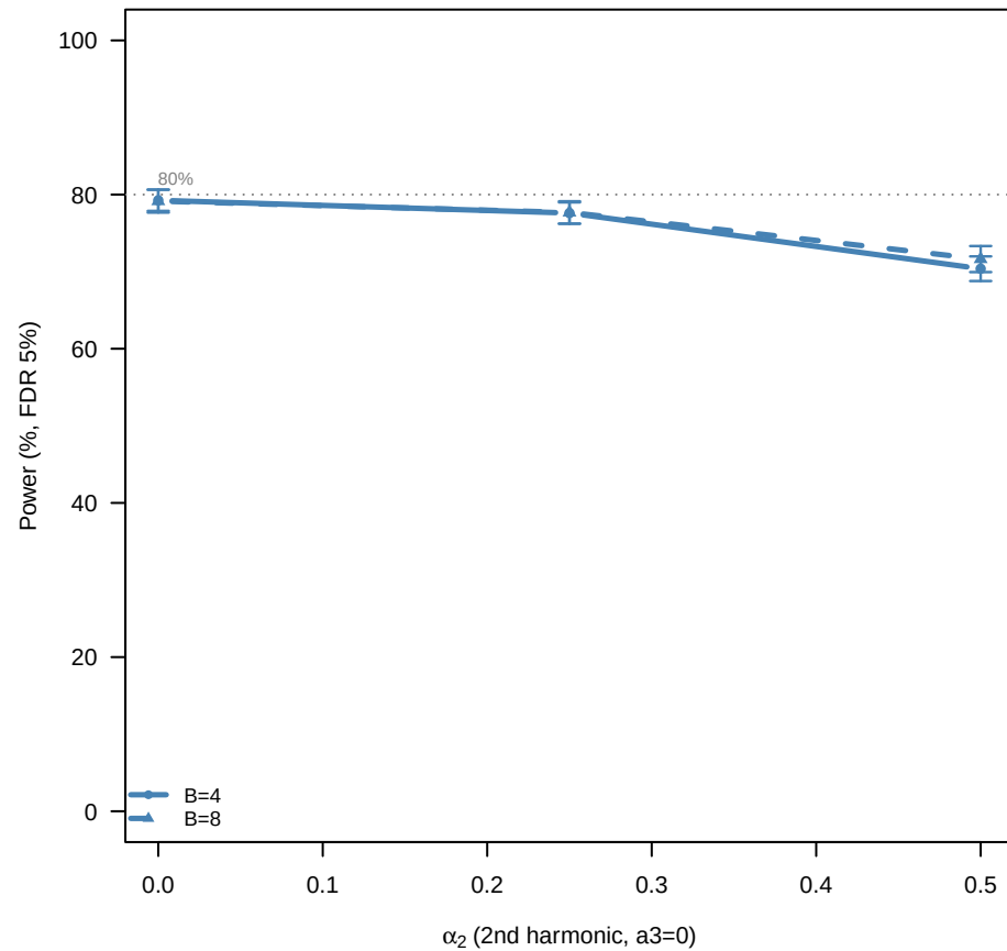
GSE54651 (r~2.9) N=24: does B protect?
