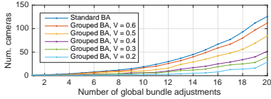
Figure 8. Number of cameras in standard and grouped BA using \gamma_r = 0.02 , S = 10 , and varying scene overlap V .
