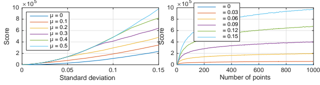
Figure 4. Next best view scores for Gaussian distributed points \mathbf{x}_j \in [0, 1] \times [0, 1] with mean \mu and std. dev. . Score S w.r.t. uniformity (left) and number of points for \mu = 0.5 (right).
