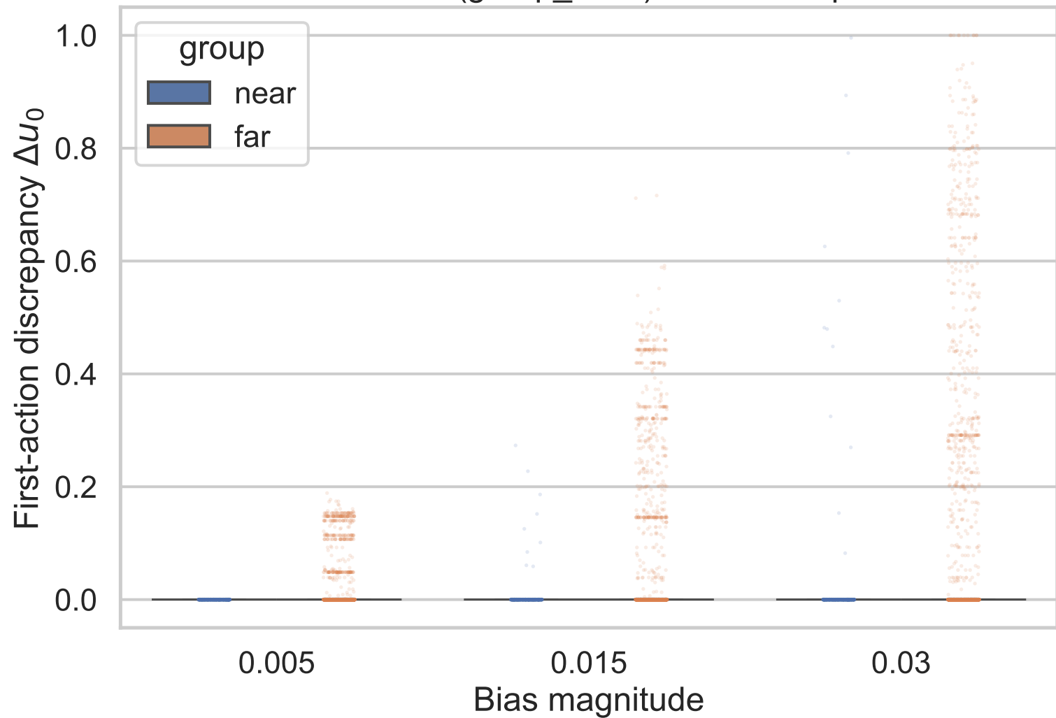
Near vs far (group_fixed) decision impact
