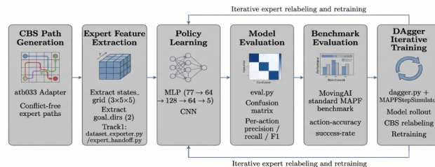
Figure 2: CBS-Based MAPF Path Planning Framework
