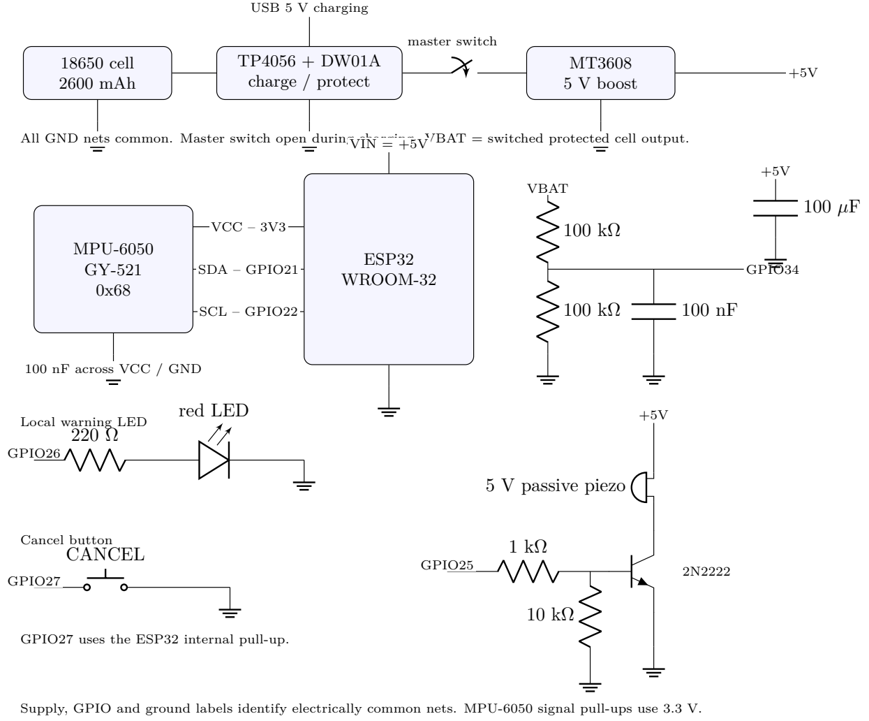
Figure 2: Complete connection-level circuit: power, sensing, battery divider, LED, transistor-driven piezo, and cancel input. The master switch is open during charging; the charger module provides no load-sharing function.
