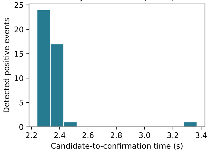
Delay distribution (n=43)
