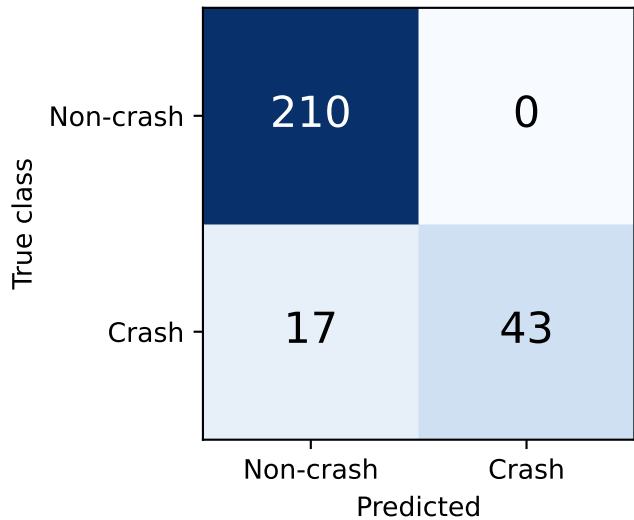
Fresh-set confusion matrix
