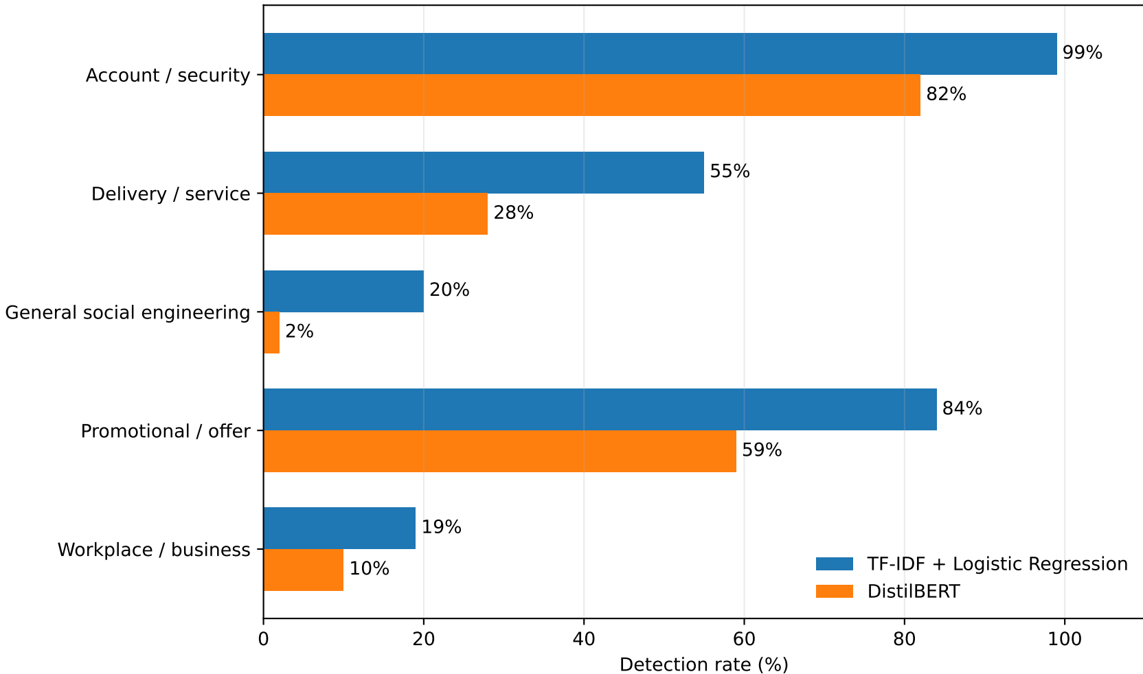
Synthetic Detection Rate by Communication Style
