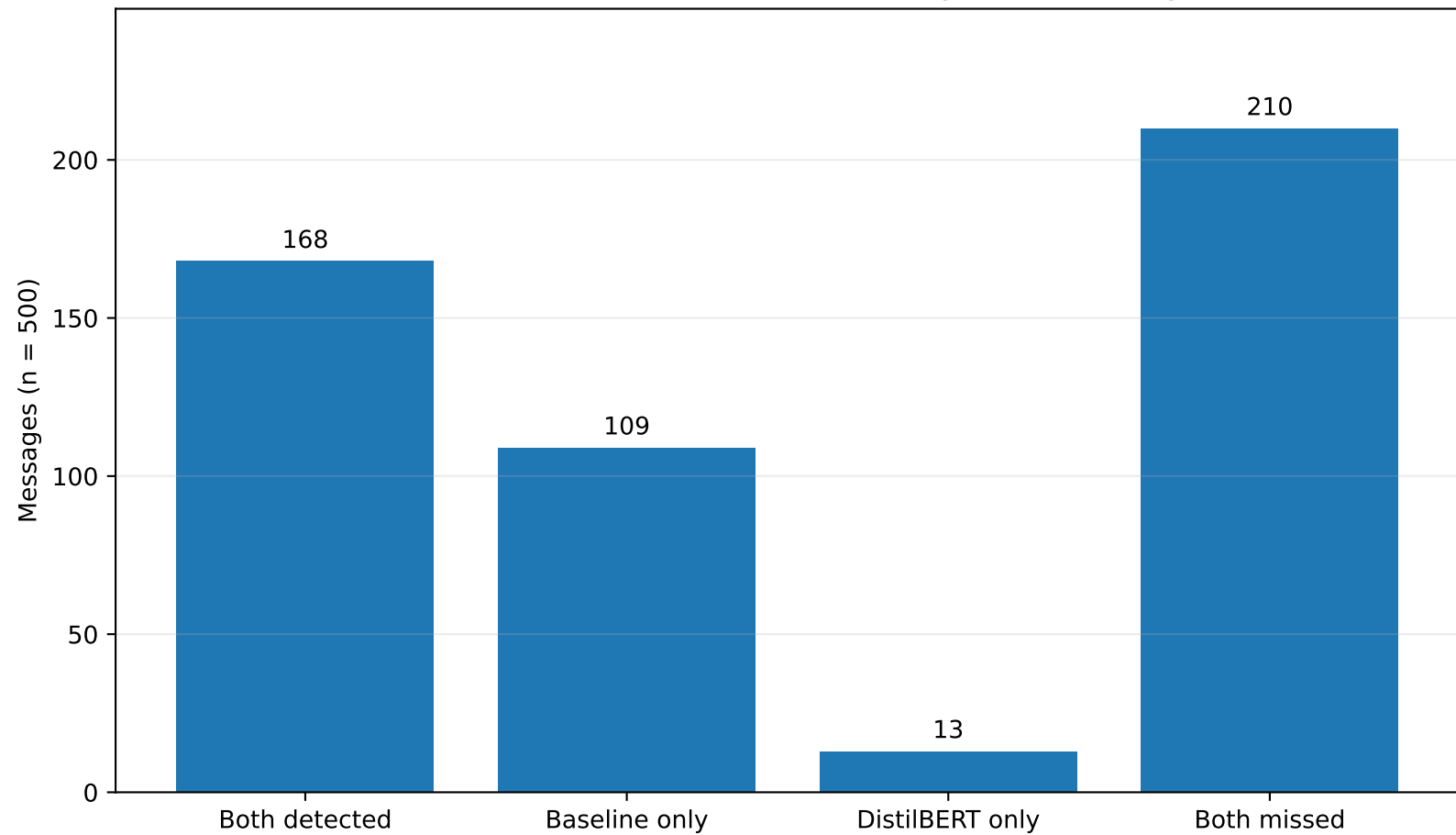
Paired Model Outcomes on Controlled Synthetic Messages
