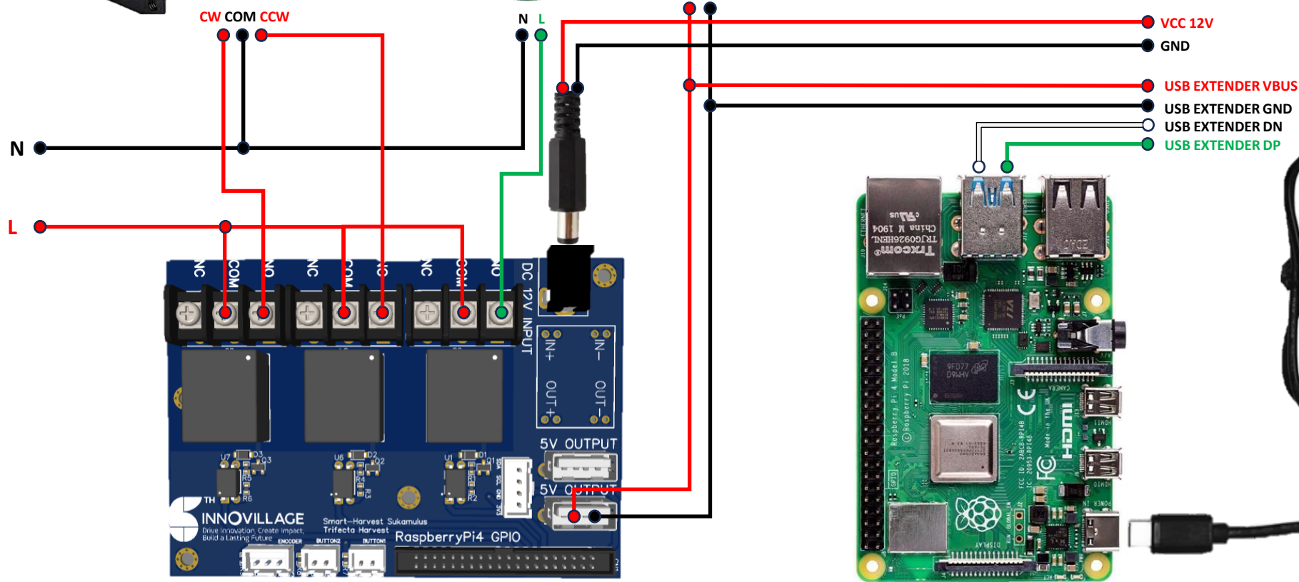
RELAY CONTROL BOARD
