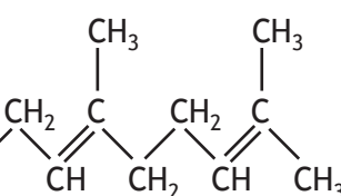
geranyl acetate
