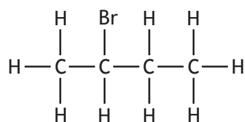
2-bromobutane
