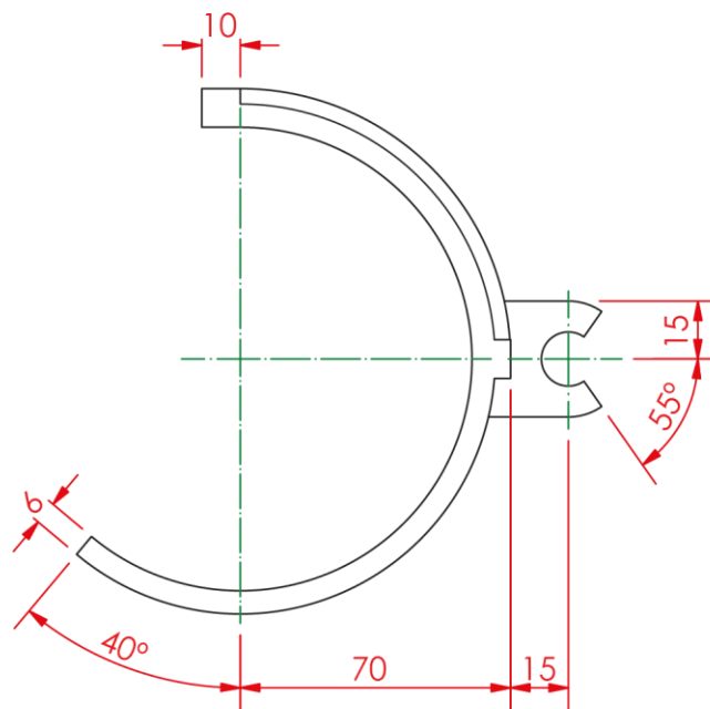
ORTHOGRAHIC VIEW (END ELEVATION)
