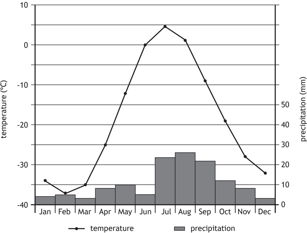
Diagram Q15A Climate graph for Isachsen, Canada (tundra)
