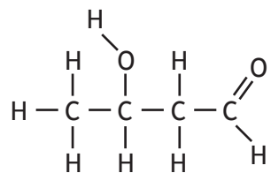
3-hydroxybutanal
