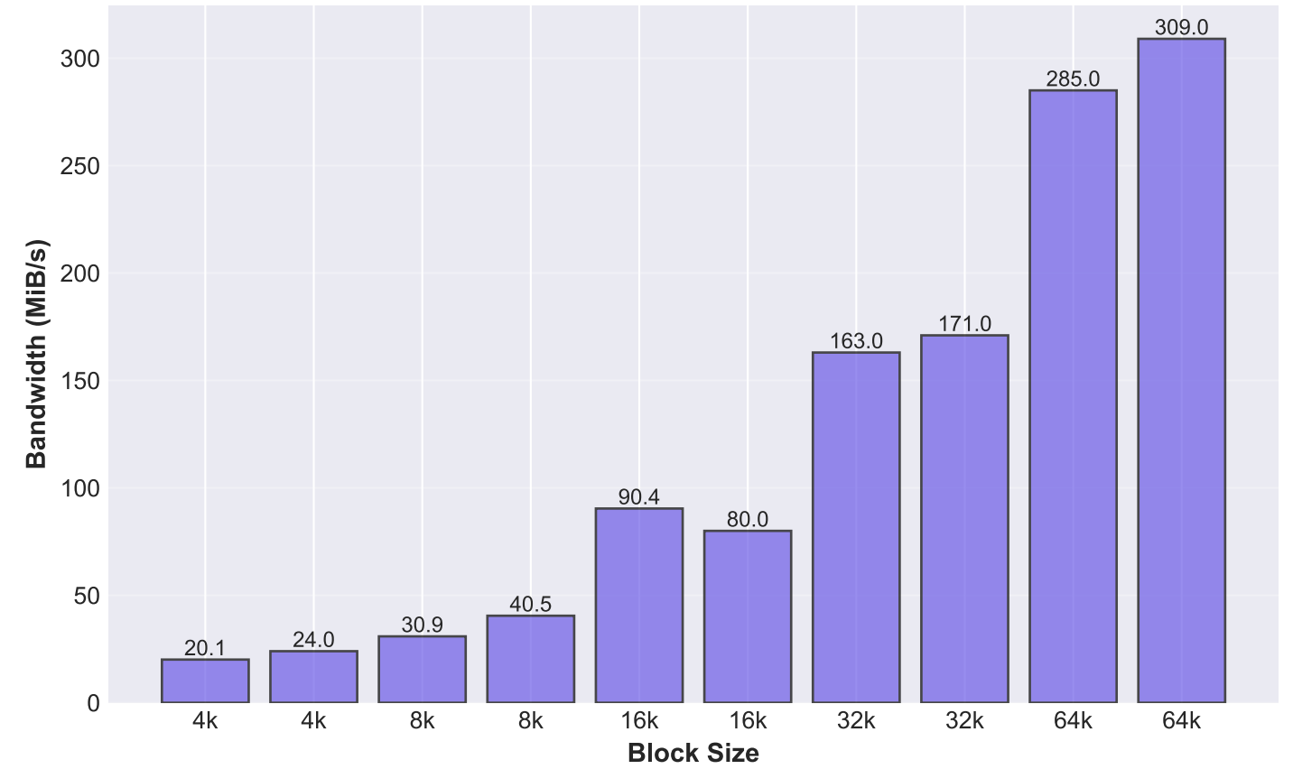
Write - Bandwidth vs Block Size
