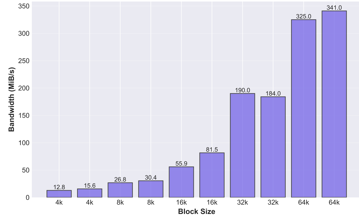
Read - Bandwidth vs Block Size
