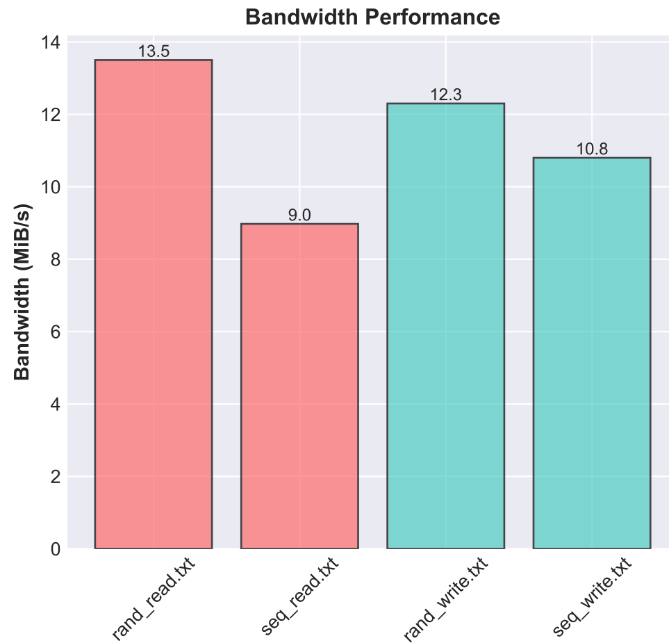
Baseline Performance Comparison (4KB, 1 Job, Depth 1)
