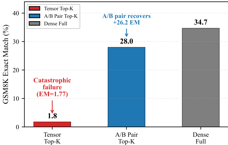
(a) Math Reasoning (GSM8K)
