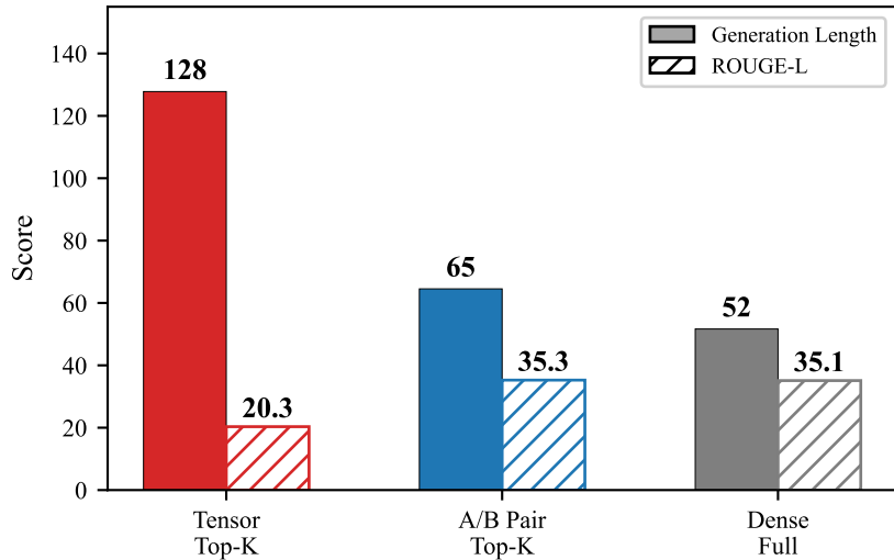
(b) Instruction Generation (Dolly-15K)
