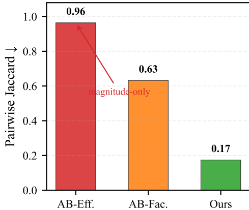
(a) Overlap
