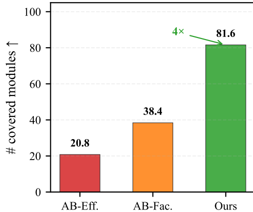
(b) Coverage
