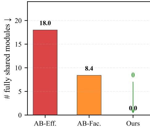
(c) Redundancy
