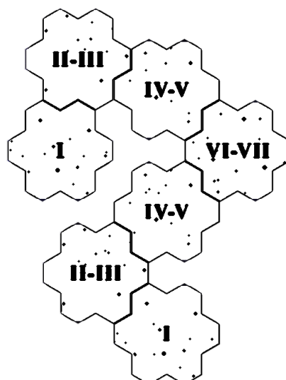
2-PLAYER SCENARIO
