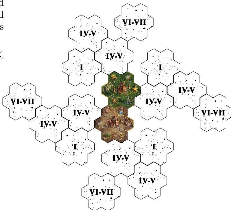
4-PLAYER SCENARIO
