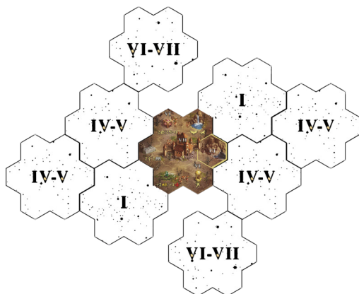
2-PLAYER SCENARIO
