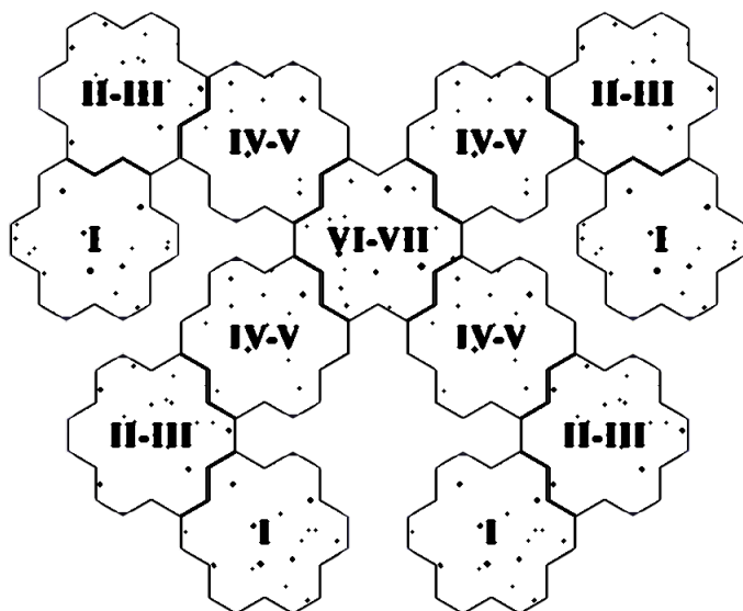
4-PLAYER SCENARIO
