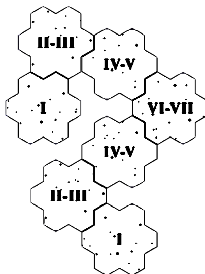
2-PLAYER SCENARIO
