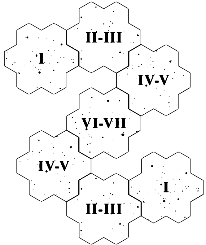
2-PLAYER SCENARIO
