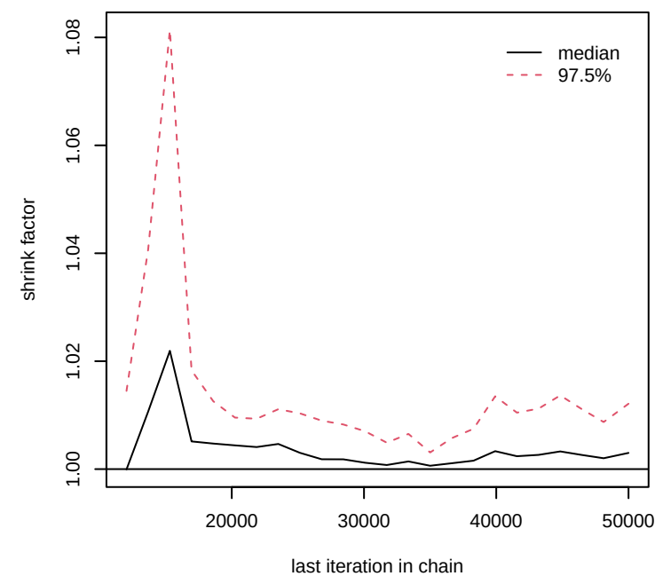
test.sens[3]
