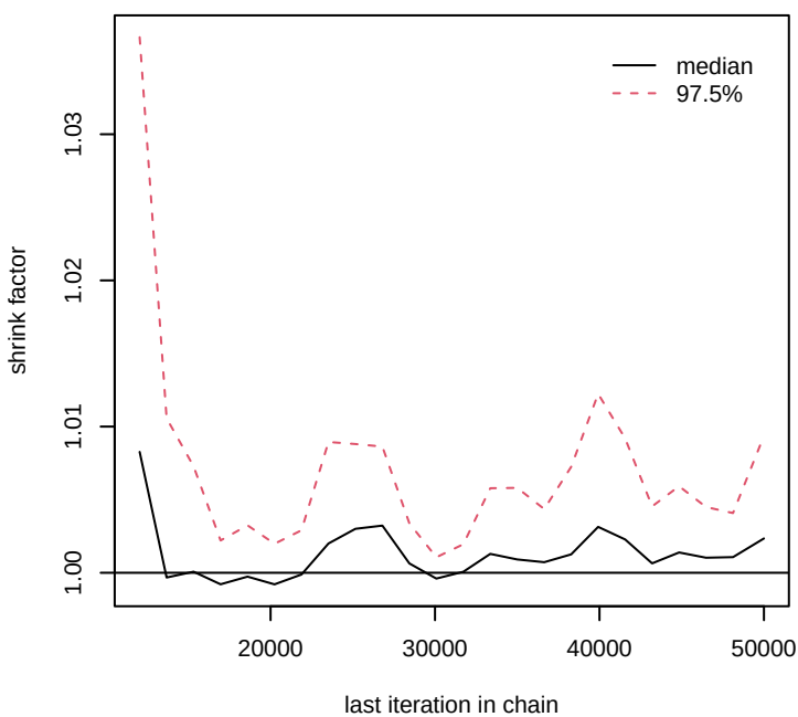
test.sens[1]
