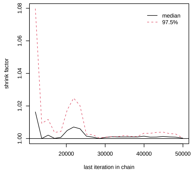
test.sens[2]
