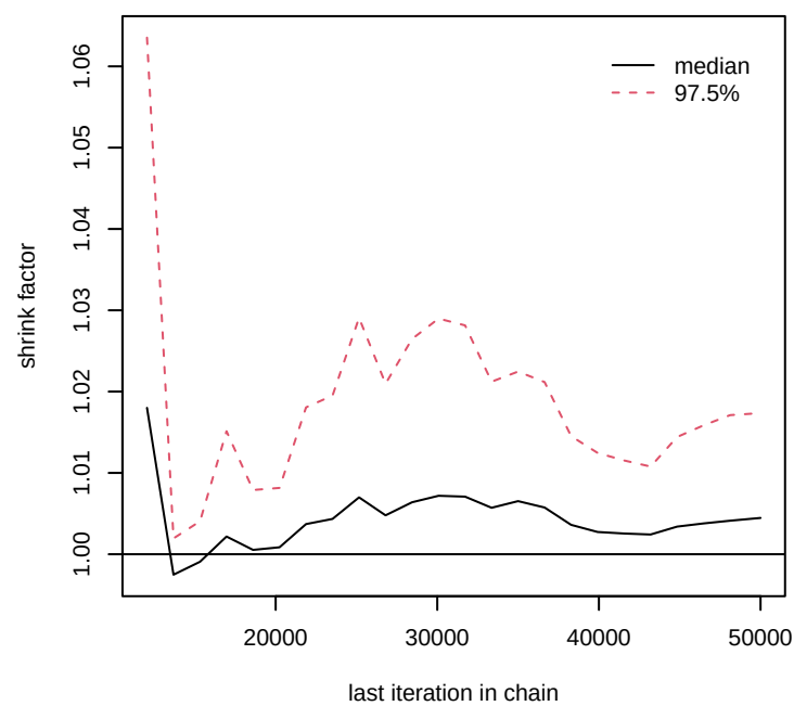
test.spec[2]
