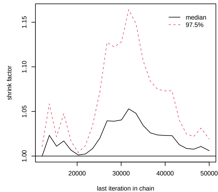
sd[2]
