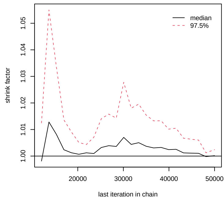
sd[1]
