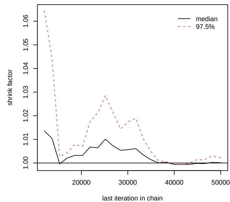
test.spec[3]
