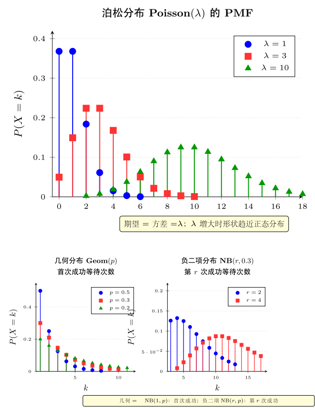
泊松 \text{Poisson}(\lambda) PMF: \lambda = 1, 3, 10
