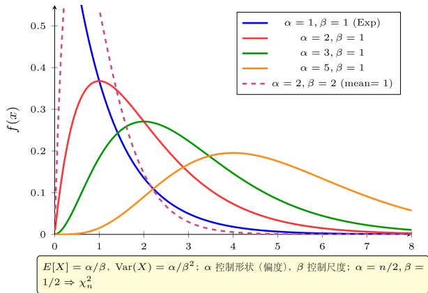
Gamma( \alpha, \beta ) 分布 PDF: f(x) = \frac{\beta^\alpha}{\Gamma(\alpha)} x^{\alpha-1} e^{-\beta x}
