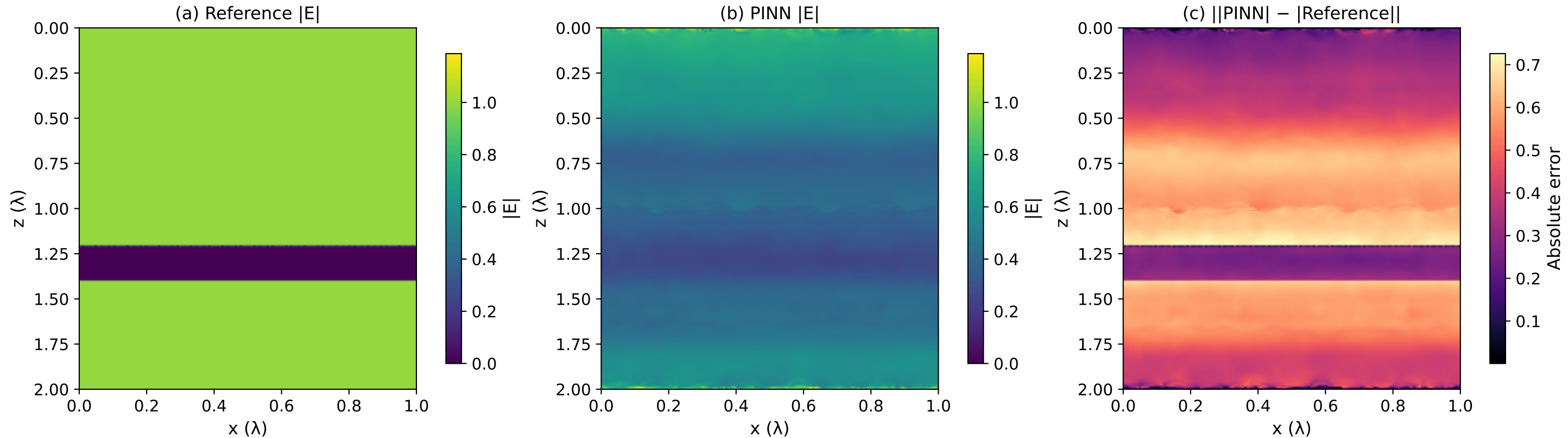
PINN vs. Reference — Field Magnitude Comparison
