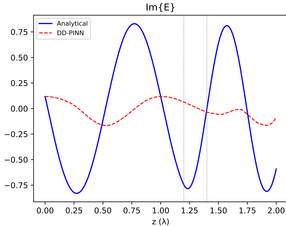
Layered benchmark (DD-PINN) L2_mag=5.078e-01
