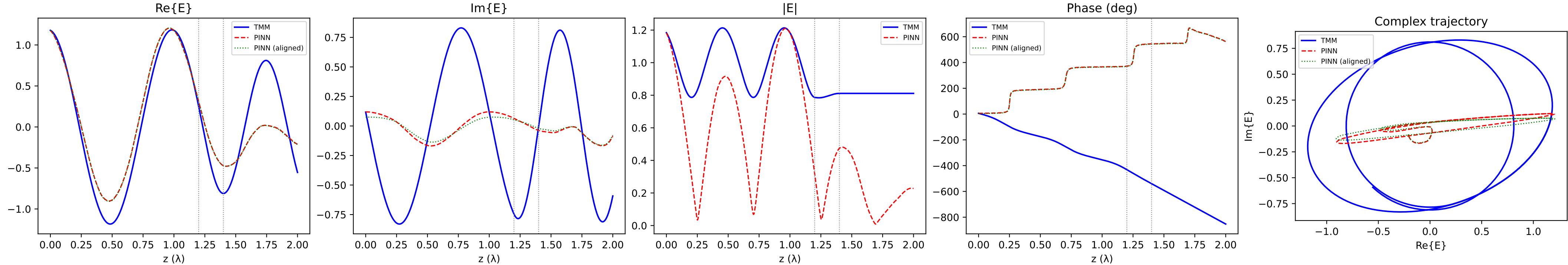
Helmholtz DD \text{complex\_L2}=6.996\text{e-}01
