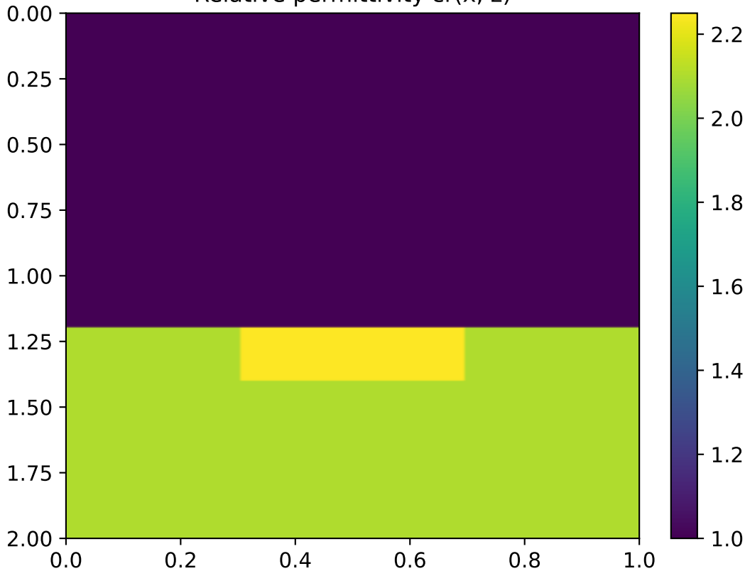
Relative permittivity \epsilon_r(x, z)
