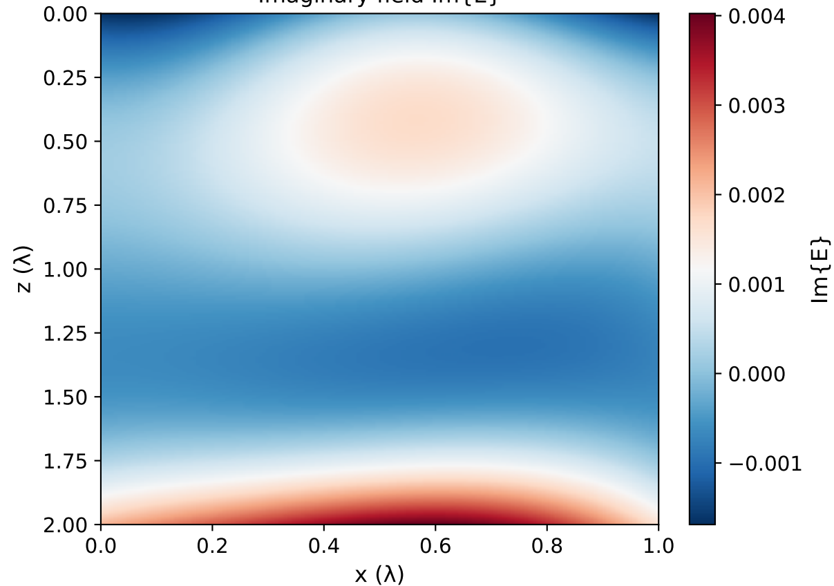
Imaginary field \text{Im}\{E\}
