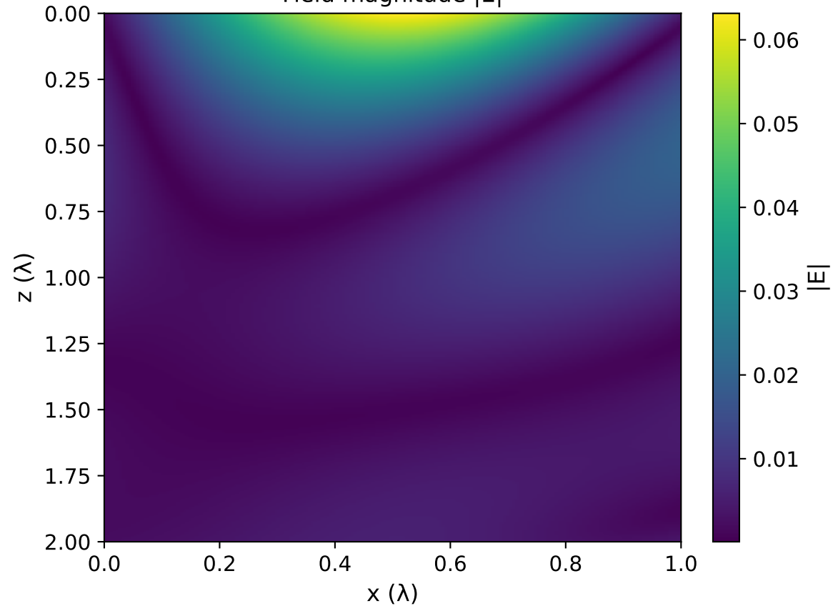
Field magnitude |E|
