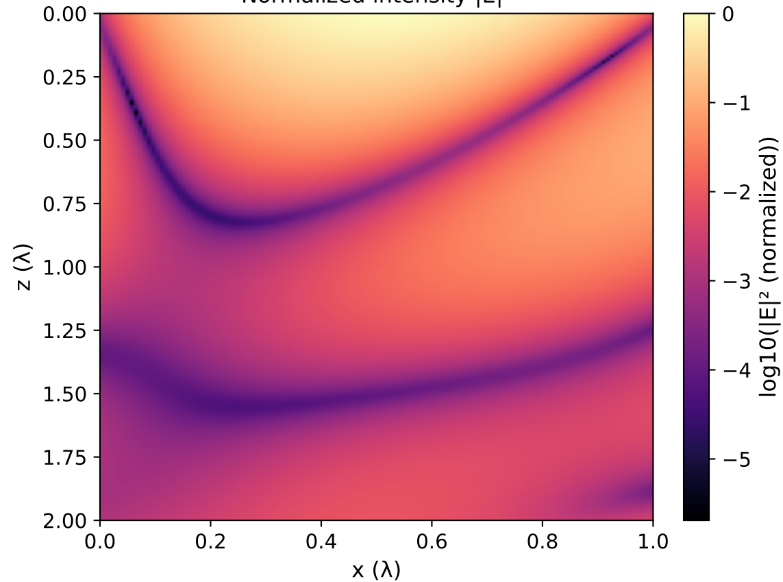
Normalized intensity |E|^2
