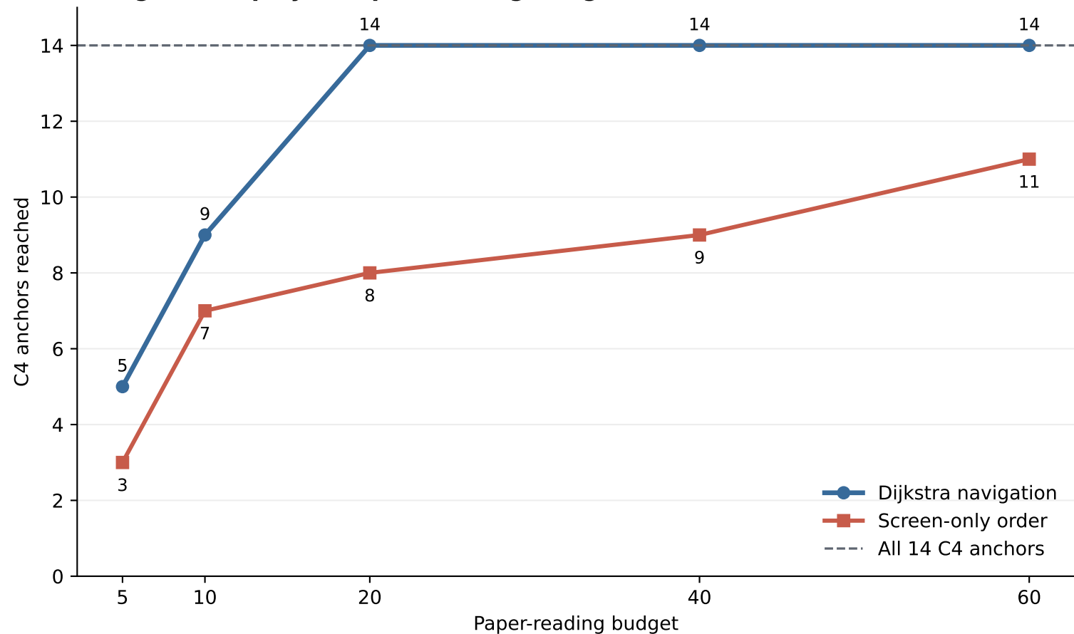
Navigation replay at equal reading budget
